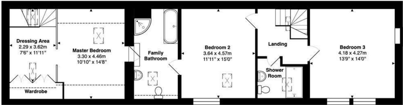
First Floor
